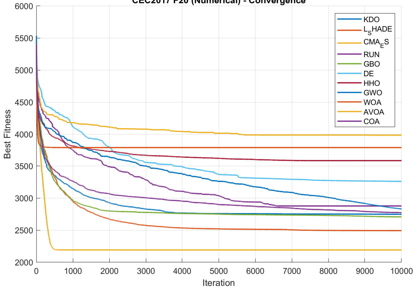
CEC2017 F20 (Numerical) - Convergence
